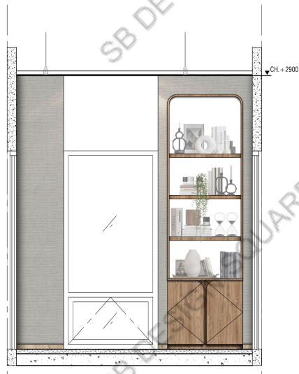
B-201 : WALL PARTITION / SHELF ELEVATION 08
