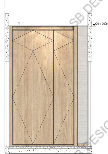
B-215 : WARDROBE ELEVATION 22
