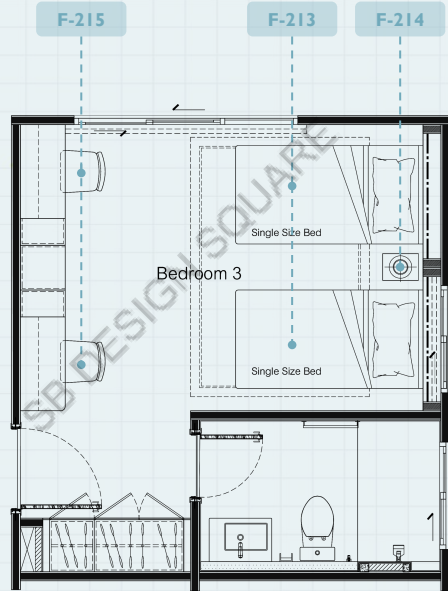
FURNITURE LAYOUT PLAN Bedroom 3
