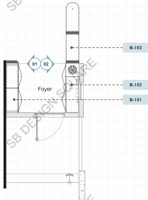
FURNITURE LAYOUT PLAN Foyer
