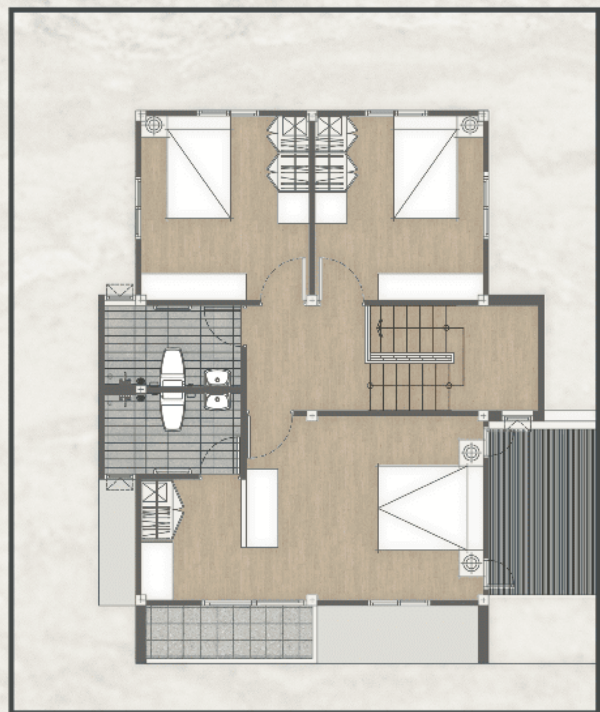
2nd Floor
